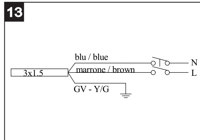
Alimentation (fig.13)
